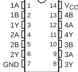
SN54HC03 . . . J OR W PACKAGE SN74HC03 . . . D, N, NS, OR PW PACKAGE (TOP VIEW)
