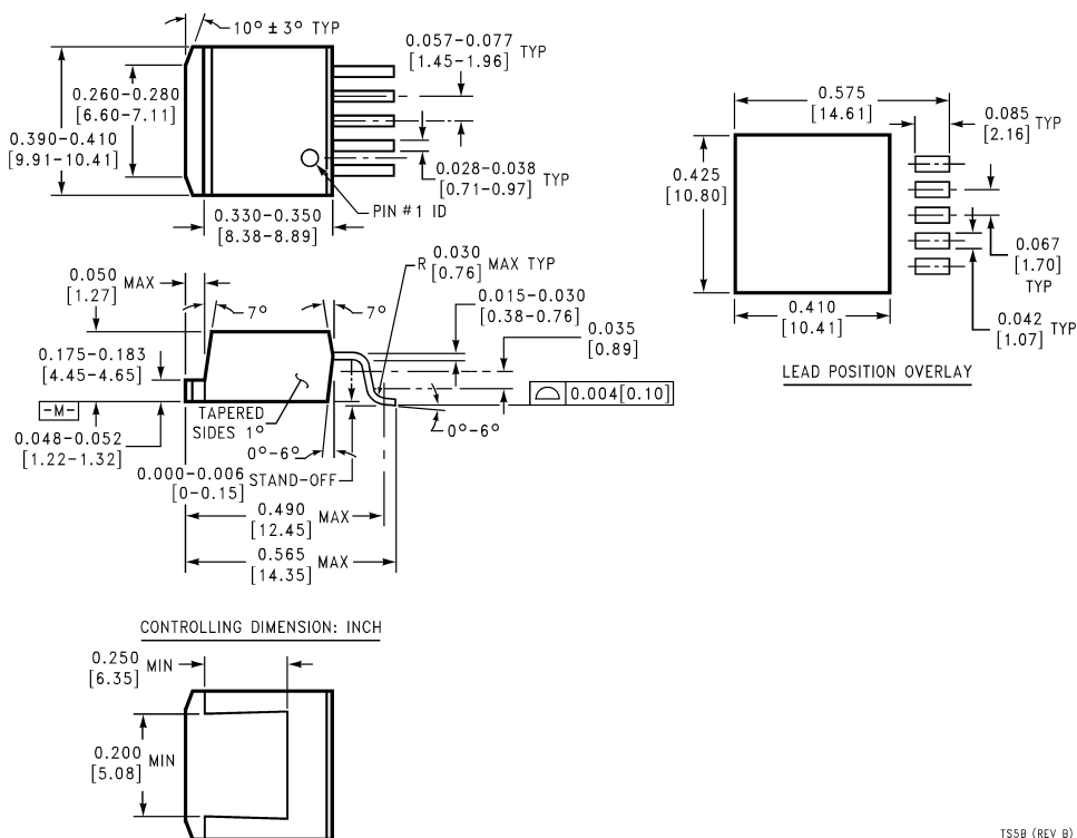
5-Lead TO-263 (S) Order Number LM2577S-12, LM2577S-15 or LM2577S-ADJ NS Package Number TSSB
